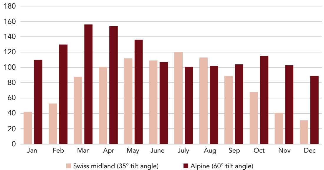
Diagram: During the winter months, alpine solar plants generate significantly higher power volumes than solar plants in the Midlands. Source: ZHAW Wädenswil
