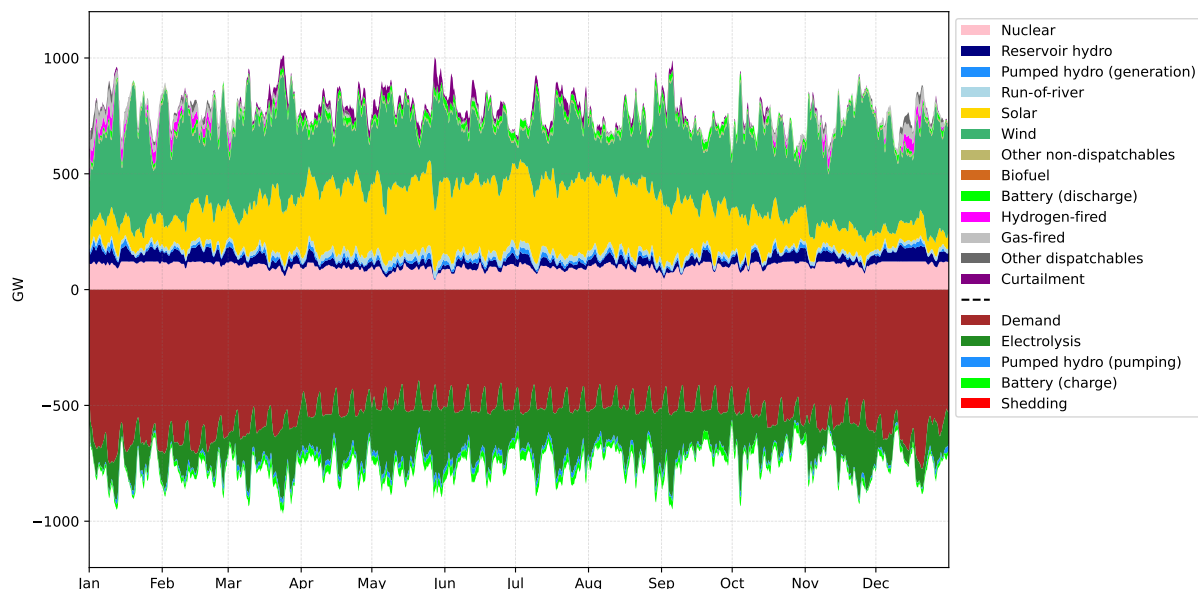
Figure 4.10.1: Annual energy dispatch (daily average) in Europe under the market-integrated conditions with the TYNDP scenario. The RES+Gas scenario in Switzerland is used for illustrative purposes.
