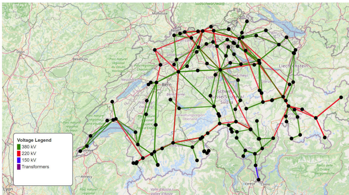
Figure 4.12.1: Topology of the Swiss transmission grid used in this study
