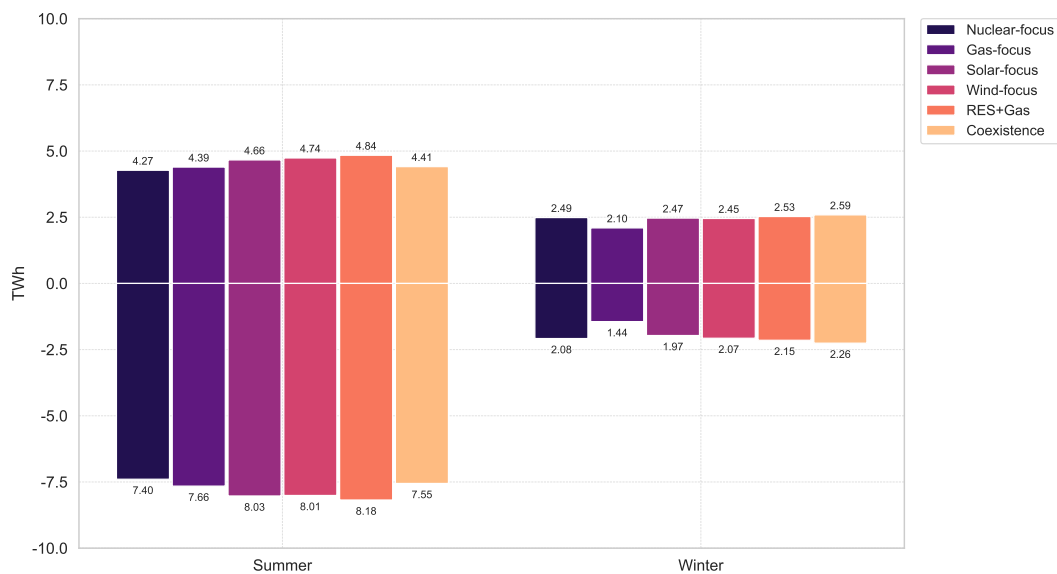
Figure 4.6.1: Seasonal generation (positive values) and pumping (negative values) of PHS plants in Switzerland under the market-integrated scenarios. Generation shows the energy after all efficiency losses, i.e. the net amount of energy injected into the system. Pumping shows the energy before any efficiency losses, i.e. the net amount of energy extracted from the system.
