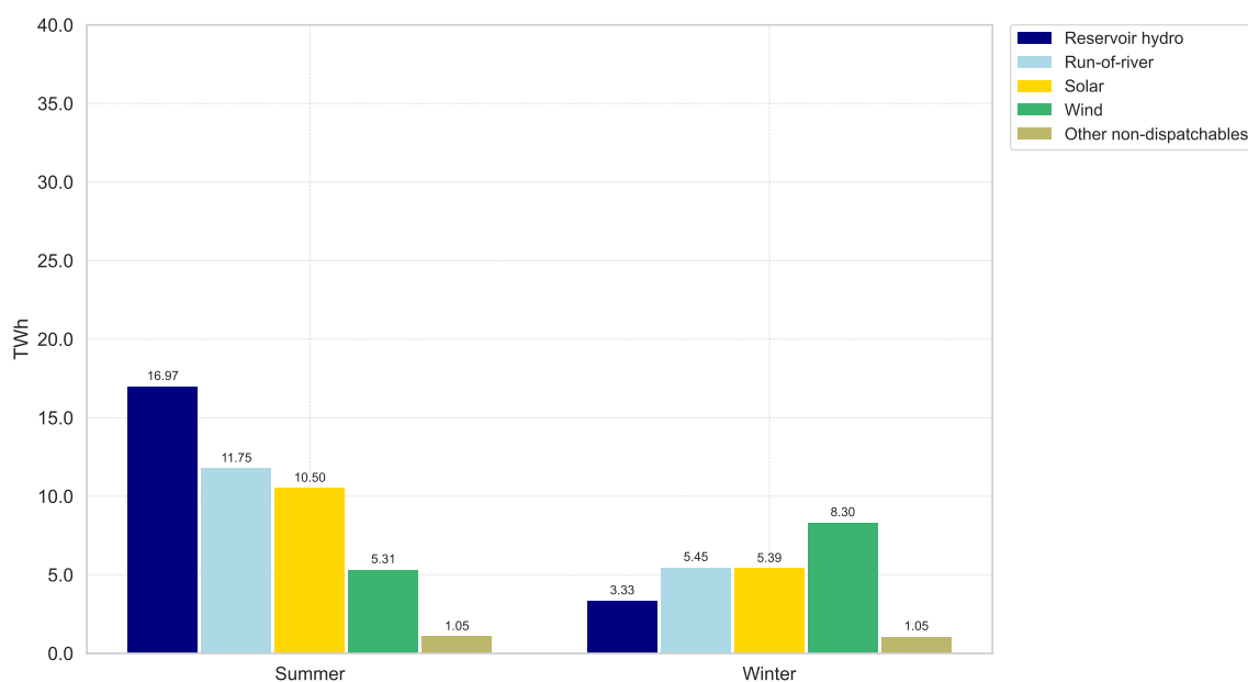
Figure 4.8.2: Seasonal renewable energy supply and hydro inflow in Switzerland in the Wind-focus scenario.
