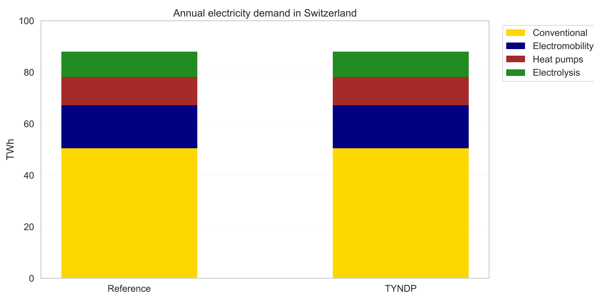
Figure 3.1.2: Final annual electricity demand in Switzerland in 2050 in the six Axpo scenarios.
