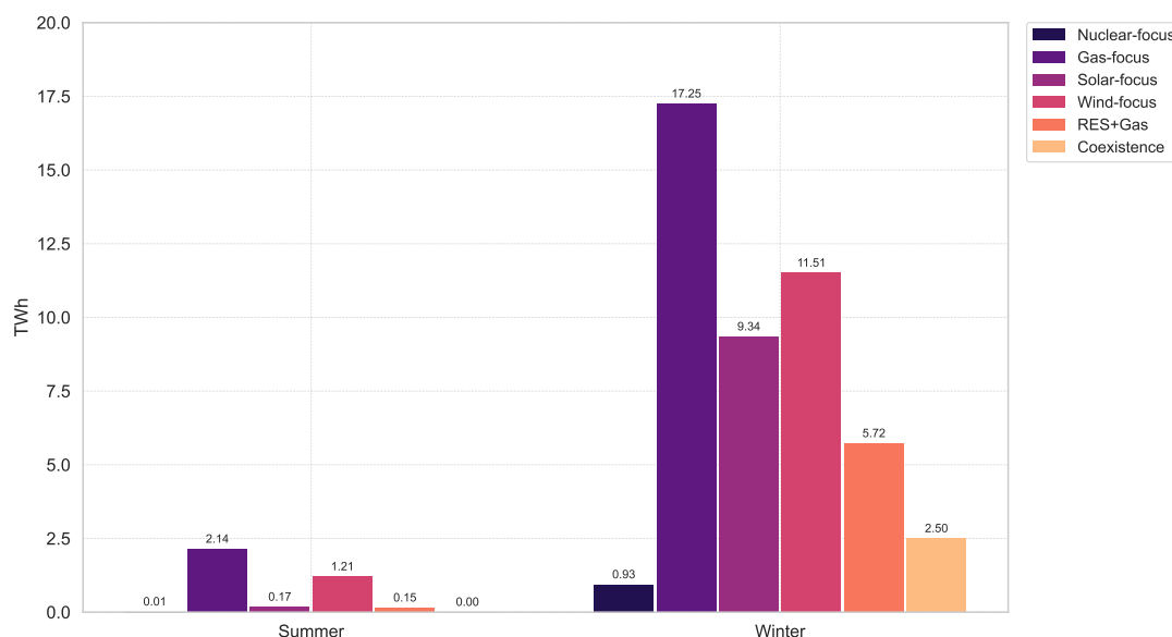
Figure 4.9.1: Seasonal gas-fired plants production in the quasi-autarky scenarios.
