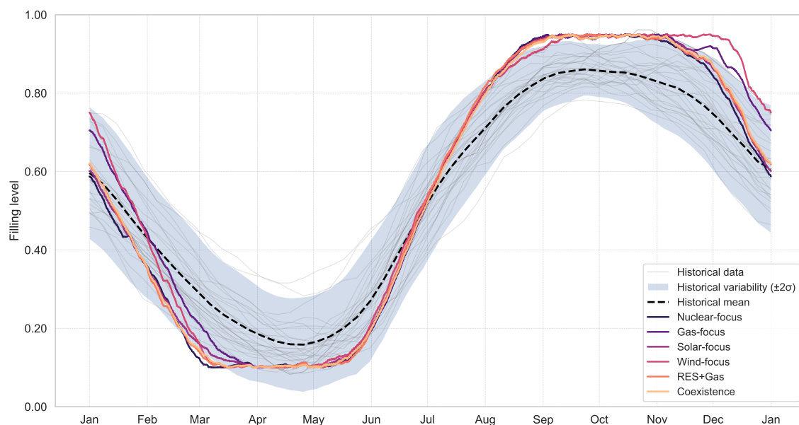
Figure 4.4.3: Reservoir storage filling levels under the quasi-autarky scenarios. Historical data are adapted from the ones available in [10].
