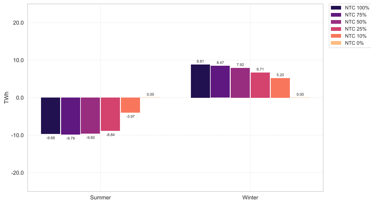
Figure 4.11.6: Seasonal net imports for the RES+Gas scenario with reduced NTCs.
