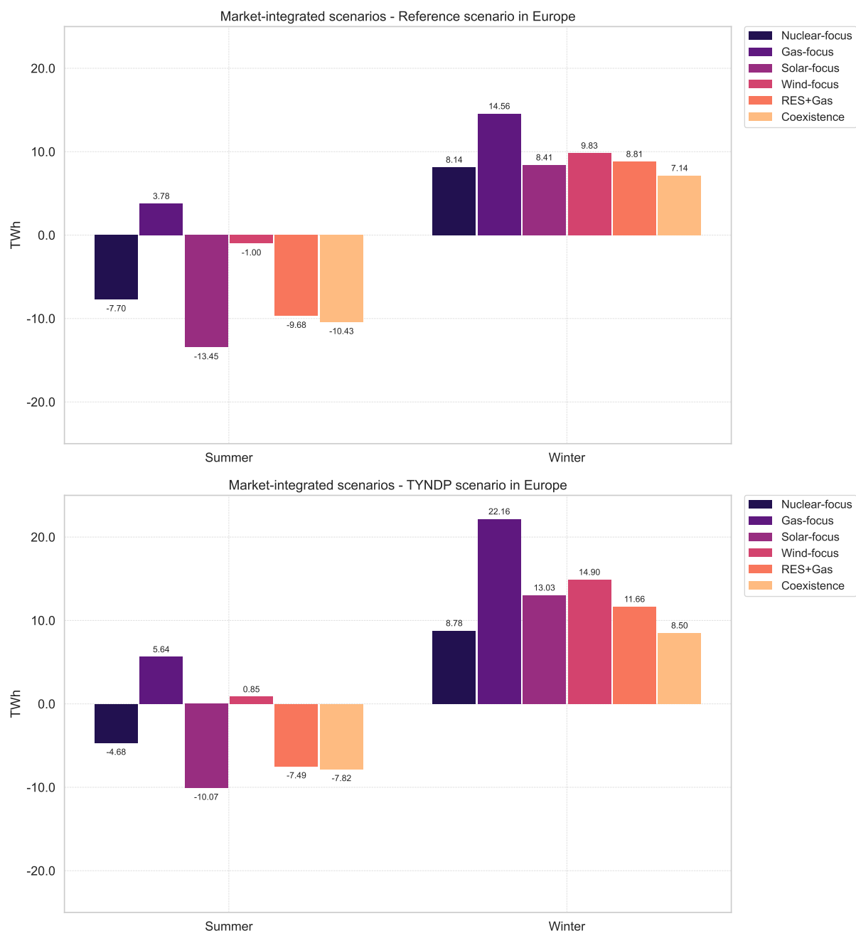
Figure 4.10.3: Seasonal net import of electricity in Switzerland in the six scenarios under the market-integrated scenarios with the Reference scenario (above) and TYNDP scenario (below) in Europe.
