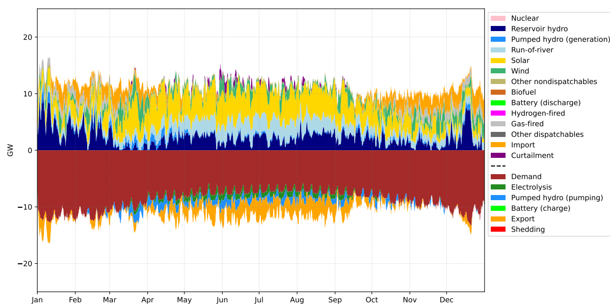
Figure 4.11.3: Annual energy dispatch (daily average) in Switzerland under the market-integrated scenario with NTCs reduced to 25%. The RES+Gas scenario in Switzerland is used for illustrative purposes.
