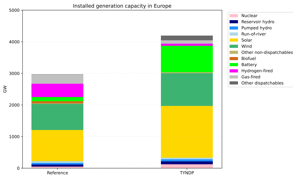
Figure 3.2.1: Installed generation capacity in Europe in 2050 in the reference Axpo scenario and the selected TYNDP scenario.
