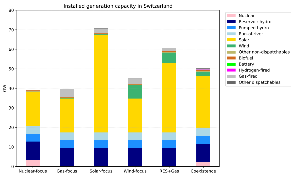
Figure 3.1.1: Installed generation capacity in Switzerland in 2050 in the six Axpo scenarios.
