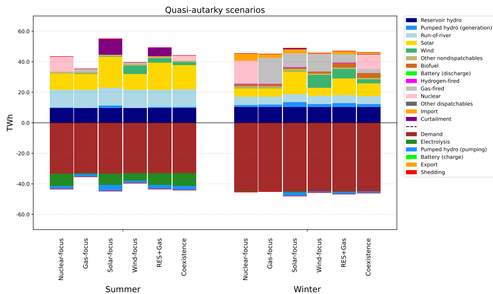
Figure 4.2.2: Seasonal electricity injections (positive values) and withdrawals (negative values) in Switzerland in the quasi-autarky simulations.
