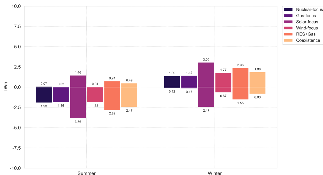
Figure 4.6.2: Seasonal generation (positive values) and pumping (negative values) of PHS plants in Switzerland under the quasi-autarky scenarios. Generation shows the energy after all efficiency losses, i.e. the net amount of energy injected into the system. Pumping shows the energy before any efficiency losses, i.e. the net amount of energy extracted from the system.
