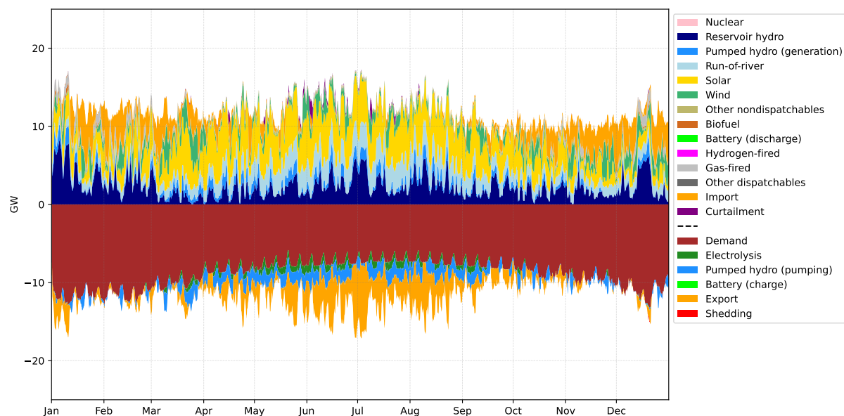
Figure 4.12.2: Annual energy dispatch (daily average) in Switzerland under the market-driven scenario with the transmission grid. The RES+Gas scenario in Switzerland is used for illustrative purposes.
