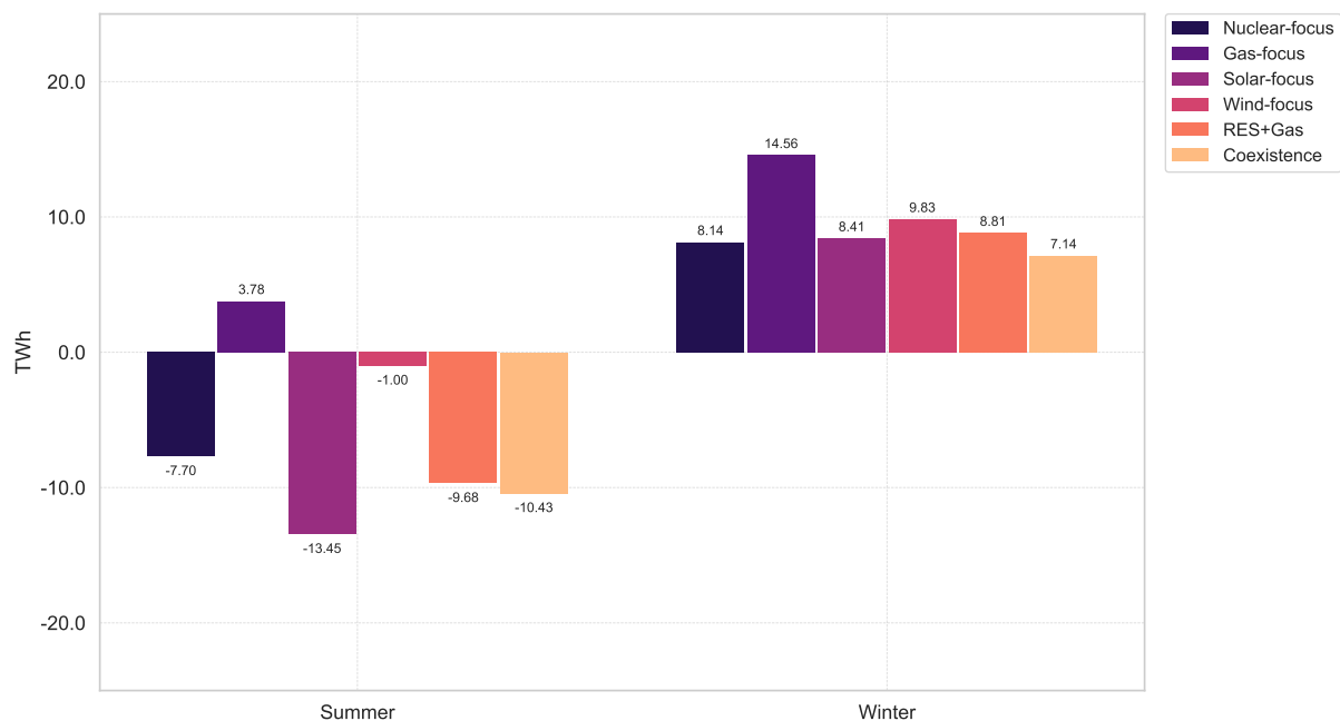
Figure 4.3.5: Seasonal net import of electricity in Switzerland under the market-integrated scenarios.
