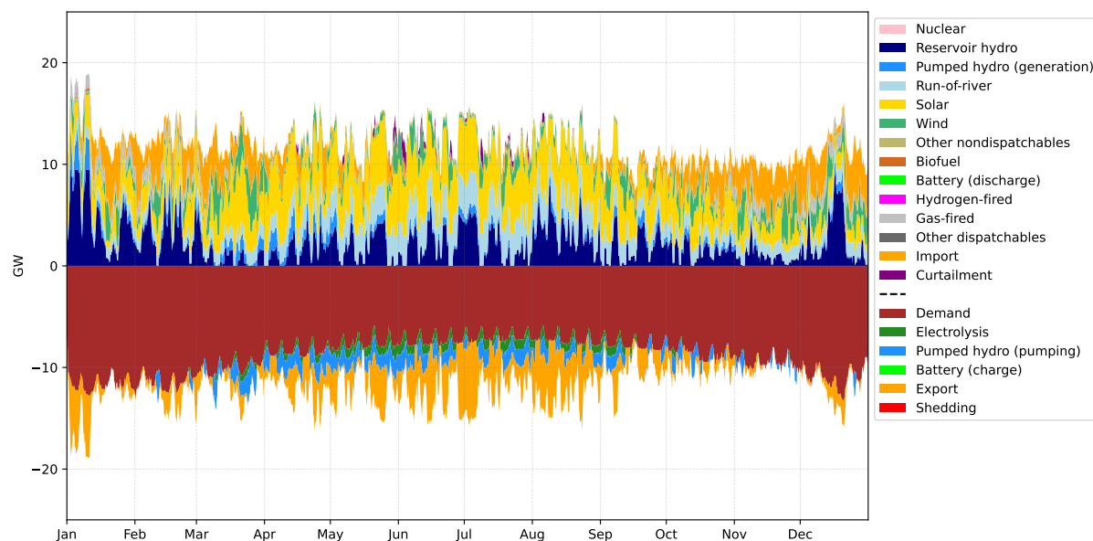
Figure 4.11.2: Annual energy dispatch (daily average) in Switzerland under the market-integrated scenario with NTCs reduced to 50%. The RES+Gas scenario in Switzerland is used for illustrative purposes.
