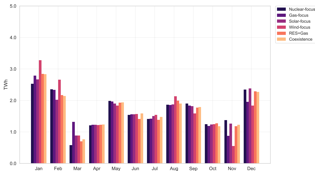
Figure 4.5.1: Monthly production of reservoir hydropower plants in Switzerland under the quasi-autarky scenarios.
