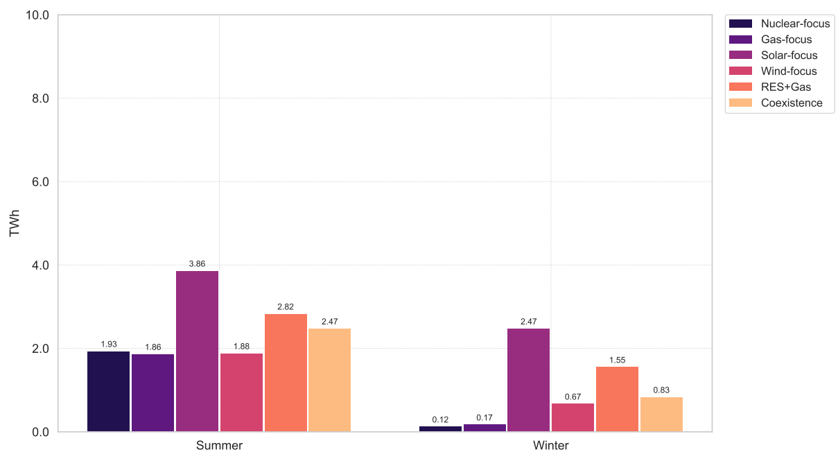
Figure 4.8.8: Seasonal pumped energy in Switzerland under the quasi-autarky scenarios.
