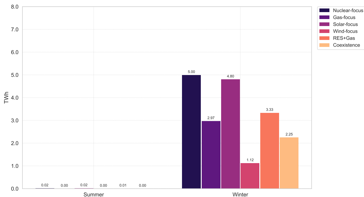
Figure 4.7.3: Seasonal net imports of electricity in Switzerland under the quasi-autarky scenarios with no flexible demand in Switzerland.
