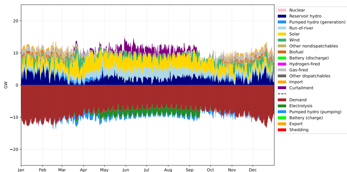
Figure 4.3.3: Annual energy dispatch (daily average) in Switzerland under the quasi-autarky scenario. The RES+Gas scenario is shown for illustrative purposes.
