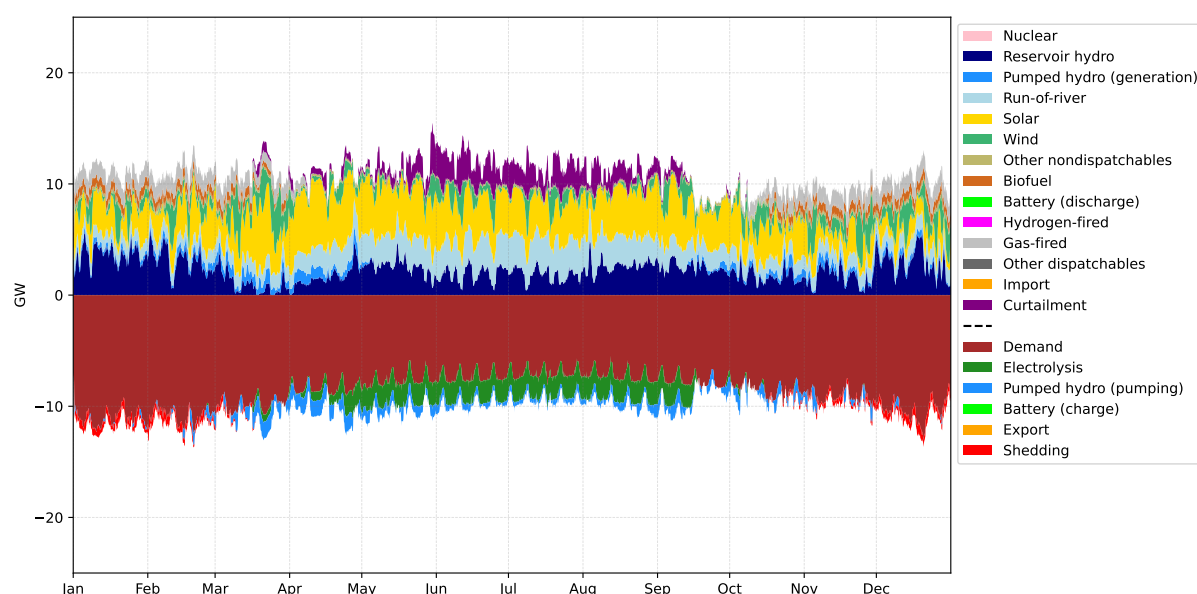
Figure 4.11.5: Annual energy dispatch (daily average) in Switzerland under the market-integrated scenario with NTCs reduced to 0%. The RES+Gas scenario in Switzerland is used for illustrative purposes.
