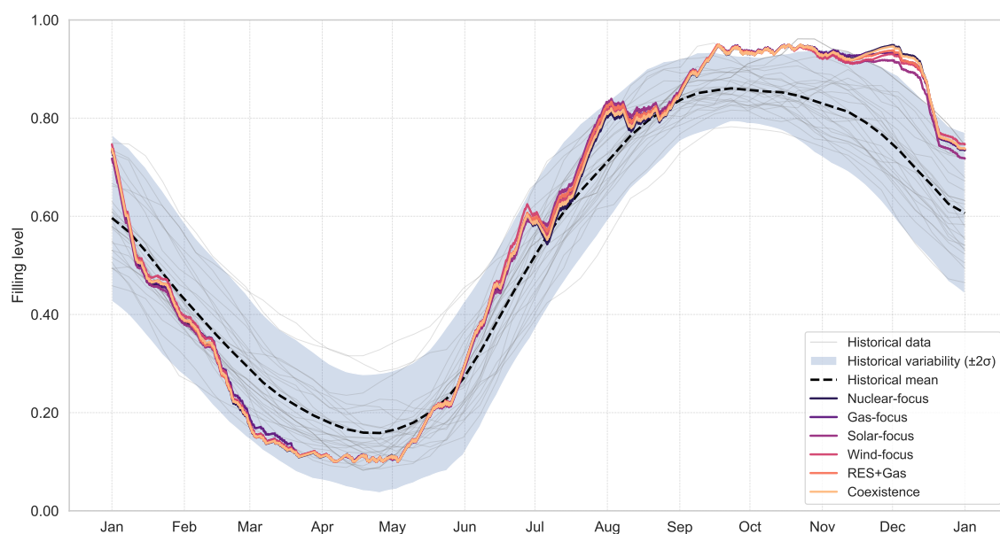
Figure 4.4.4: Reservoir storage filling levels under the market-integrated scenarios. Historical data are adapted from the ones available in [10].
