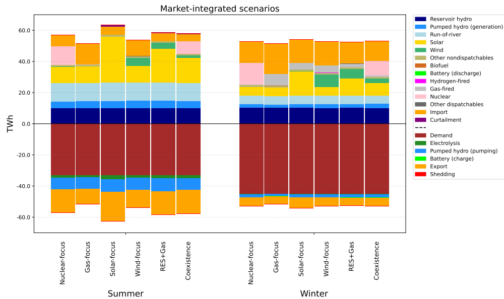
Figure 4.2.1: Seasonal electricity injections (positive values) and withdrawals (negative values) in Switzerland in the market-integrated simulations.
