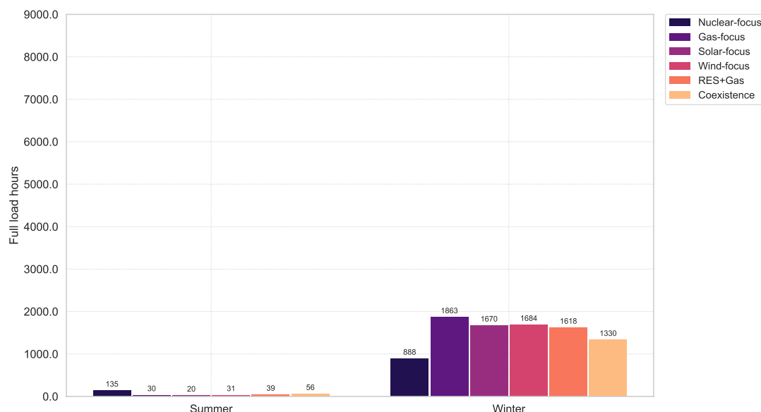
Figure 4.9.3: Seasonal equivalent full load hours of gas-fired plants (including old existing plants, new gas-fired plants, and new plants with CCS technologies) in the market-integrated scenarios.
