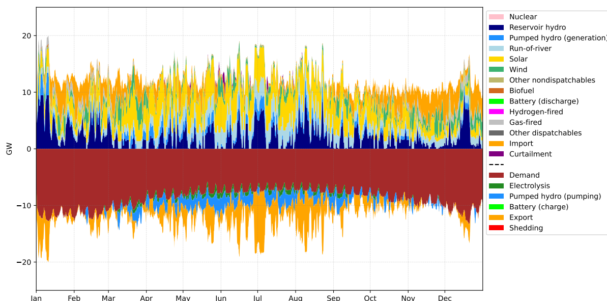
Figure 4.11.1: Annual energy dispatch (daily average) in Switzerland under the market-integrated scenario with NTCs reduced to 75%. The RES+Gas scenario in Switzerland is used for illustrative purposes.
