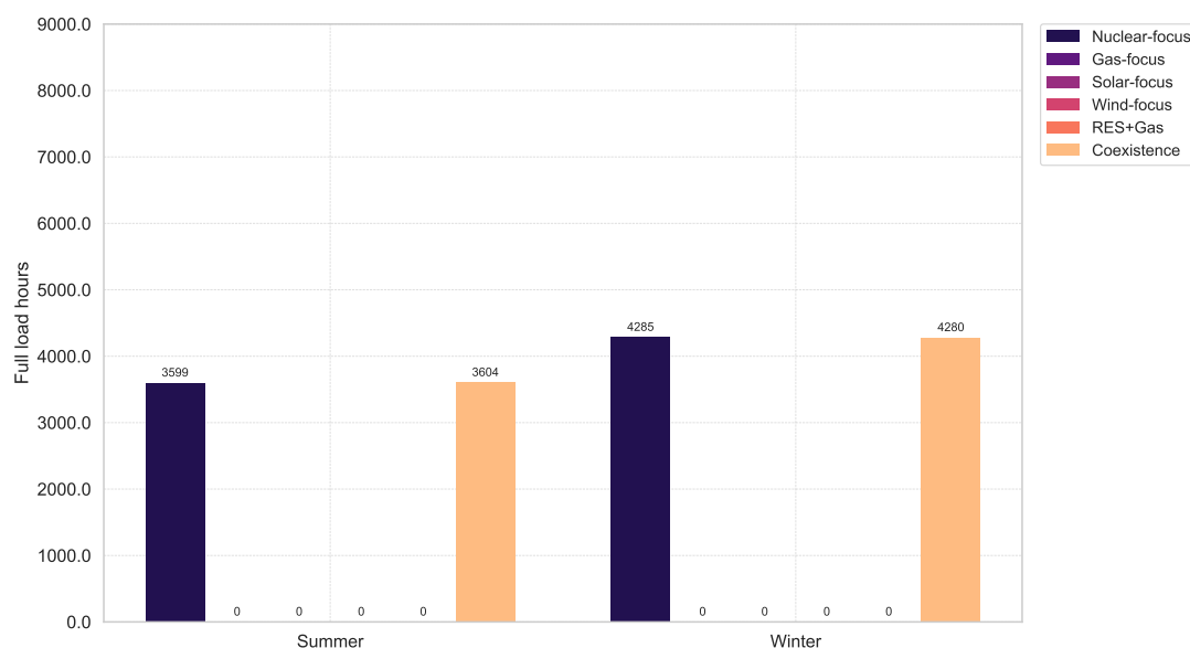
Figure 4.9.4: Seasonal equivalent full load hours of nuclear plants in the market-integrated scenarios.
