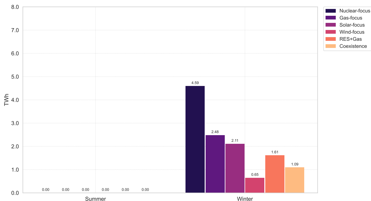
Figure 4.7.4: Seasonal net imports of electricity in Switzerland under the quasi-autarky scenarios with 2 GW (6 GWh) of batteries in Switzerland.
