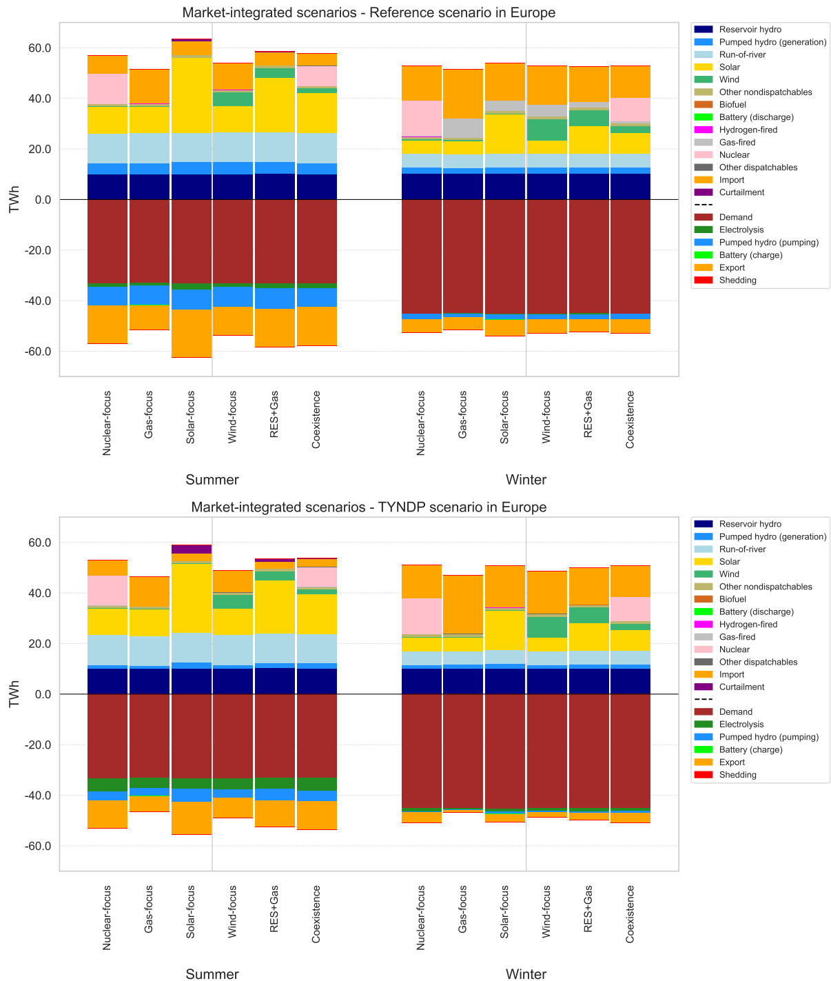
Figure 4.10.2: Seasonal injections and withdrawals in Switzerland with the Reference scenario (above) and TYNDP scenario (below) in Europe.
