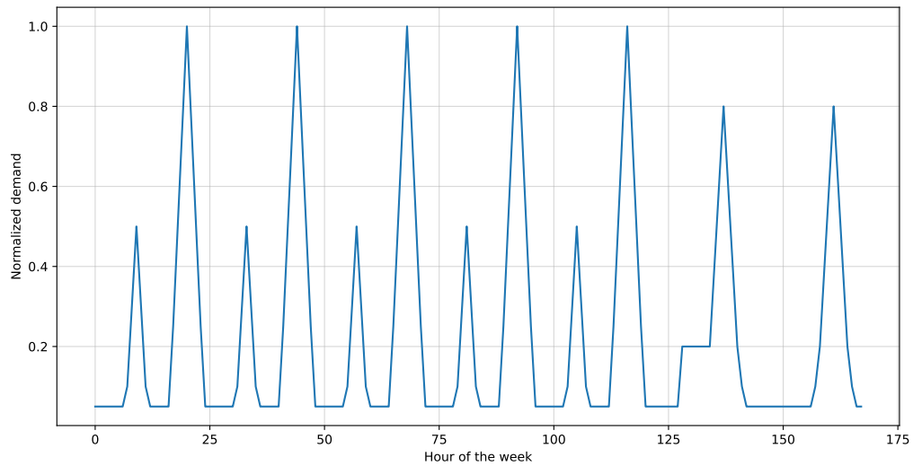
Figure A.1: Normalized electromobility demand during the first week of January (first day is a Monday).
