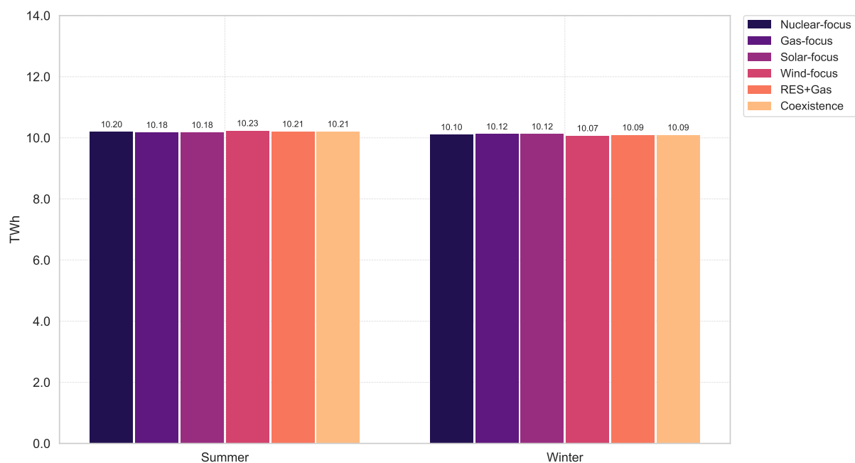
Figure 4.10.4: Seasonal production of reservoir hydropower plants in Switzerland under the TYNDP market-integrated scenarios.
