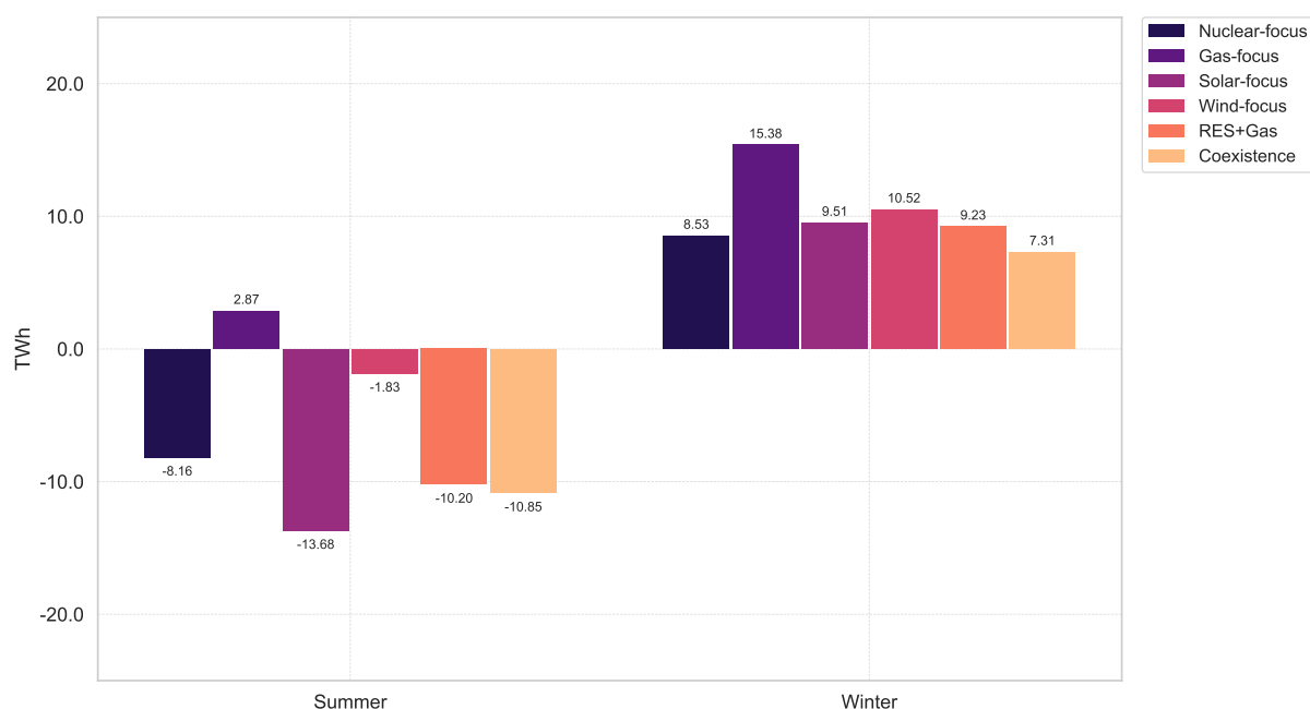
Figure 4.12.3: Seasonal net imports for the RES+Gas scenario with the transmission grid.
