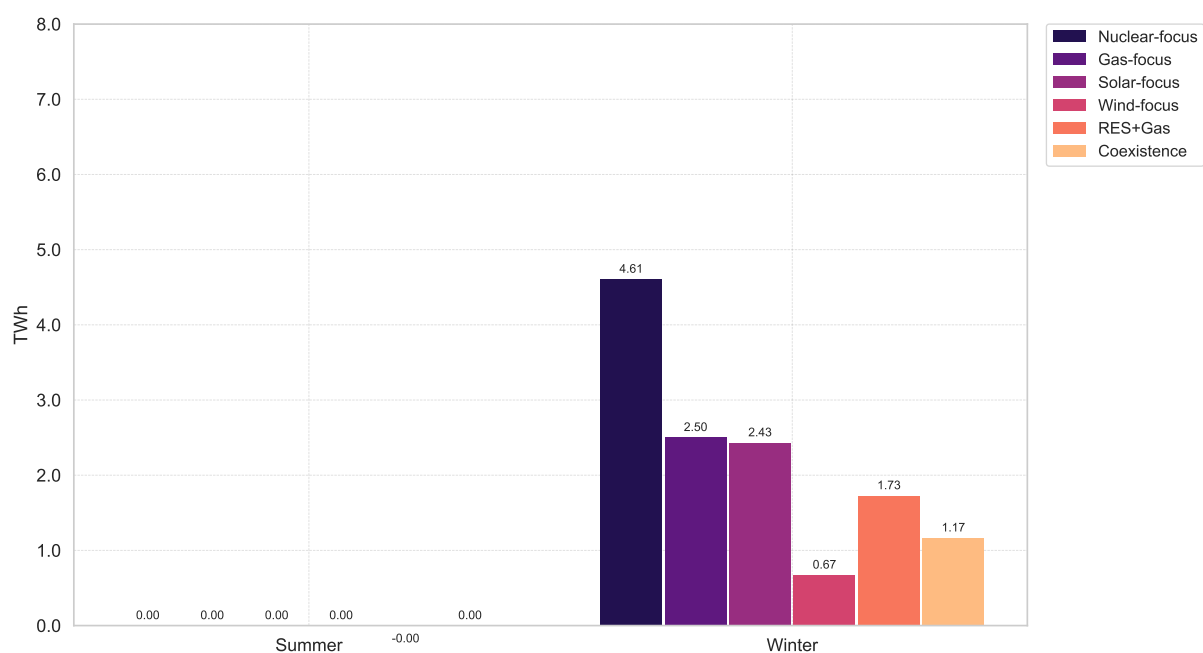
Figure 4.3.1: Seasonal net imports of electricity in Switzerland in the quasi-autarky scenarios.
