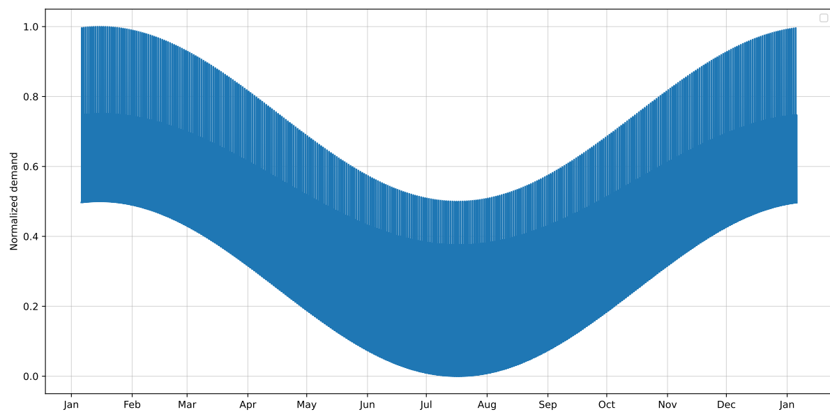
Figure A.3: Normalized heat pump demand, annual profile.
