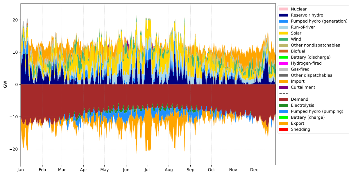
Figure 4.3.4: Annual energy dispatch (daily average) in Switzerland under the market-integrated scenario. The RES+Gas scenario is shown for illustrative purposes.
