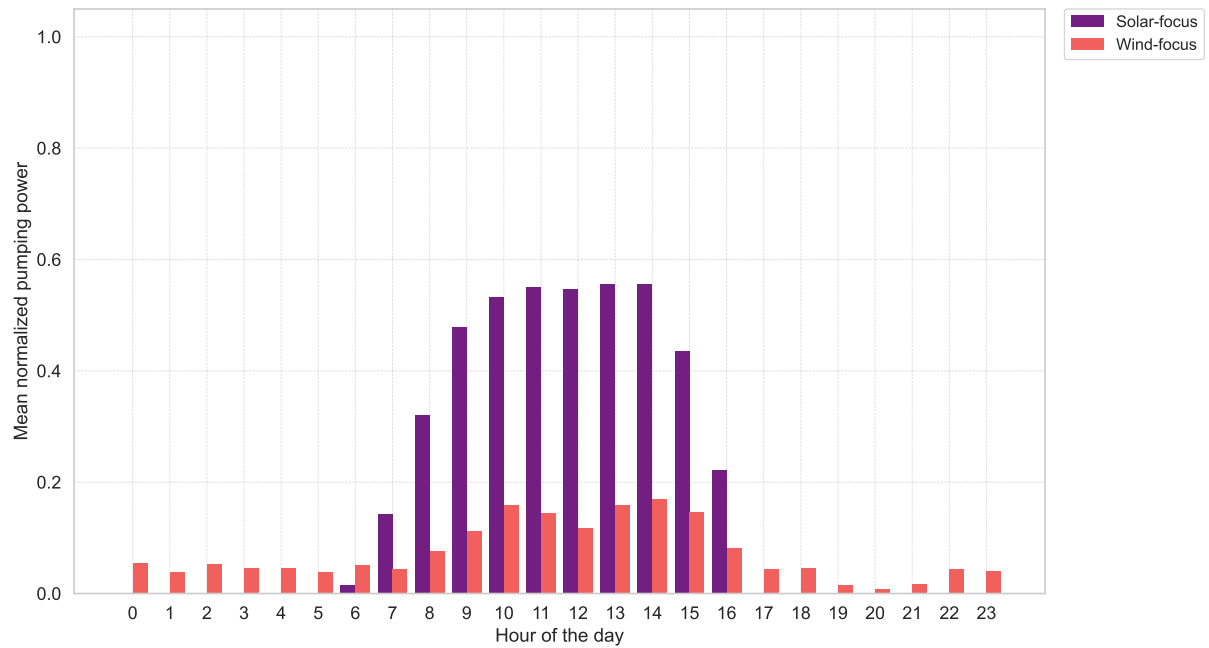
Figure 4.8.7: Mean hourly pumping power in the Solar-focus and Wind-focus quasi-autarky scenarios.
