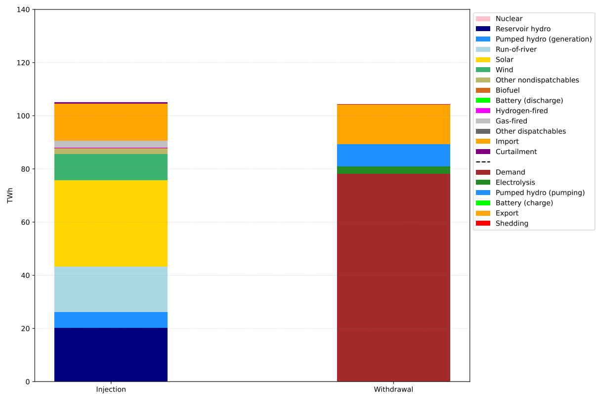
Figure 4.12.5: Annual energy dispatch (aggregated) in Switzerland under the market-driven scenario with the transmission grid included in Switzerland. The RES+Gas scenario in Switzerland is used for illustrative purposes.
