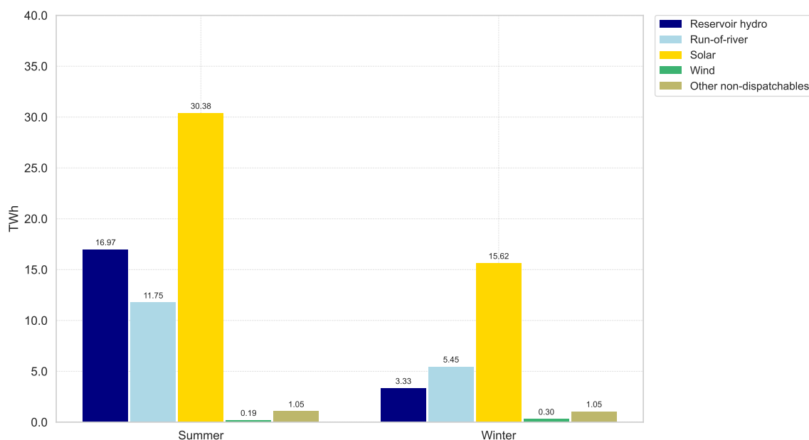
Figure 4.8.1: Seasonal renewable energy supply and hydro inflow in Switzerland in the Solar-focus scenario.
