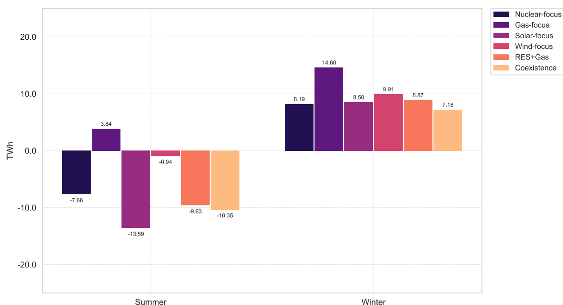
Figure 4.7.2: Seasonal net imports of electricity in Switzerland under the market-integrated scenarios with 2 GW (6 GWh) of batteries in Switzerland.
