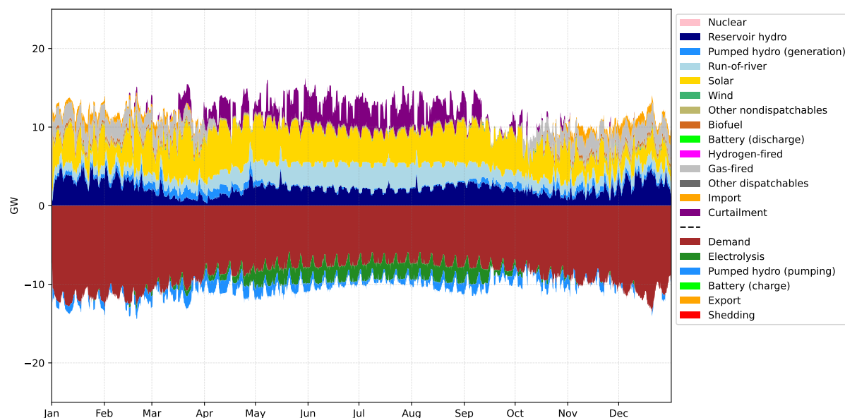
Figure 4.8.4: Annual energy dispatch (daily average) in Switzerland under the Solar-focus quasi-autarky scenario.
