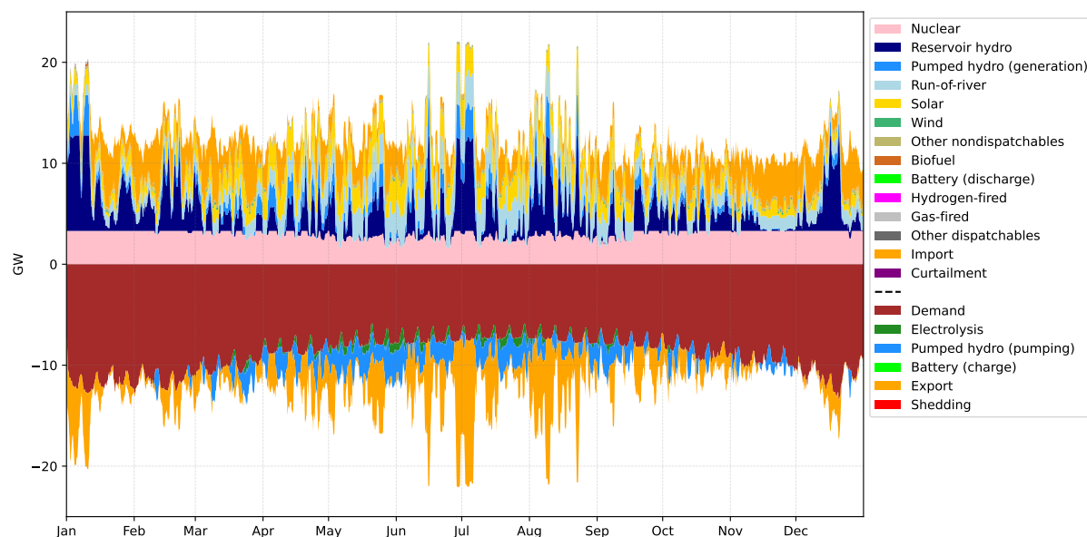
Figure 4.9.5: Annual energy dispatch (daily average) in Switzerland under the Nuclear-focus market-integrated scenario.
