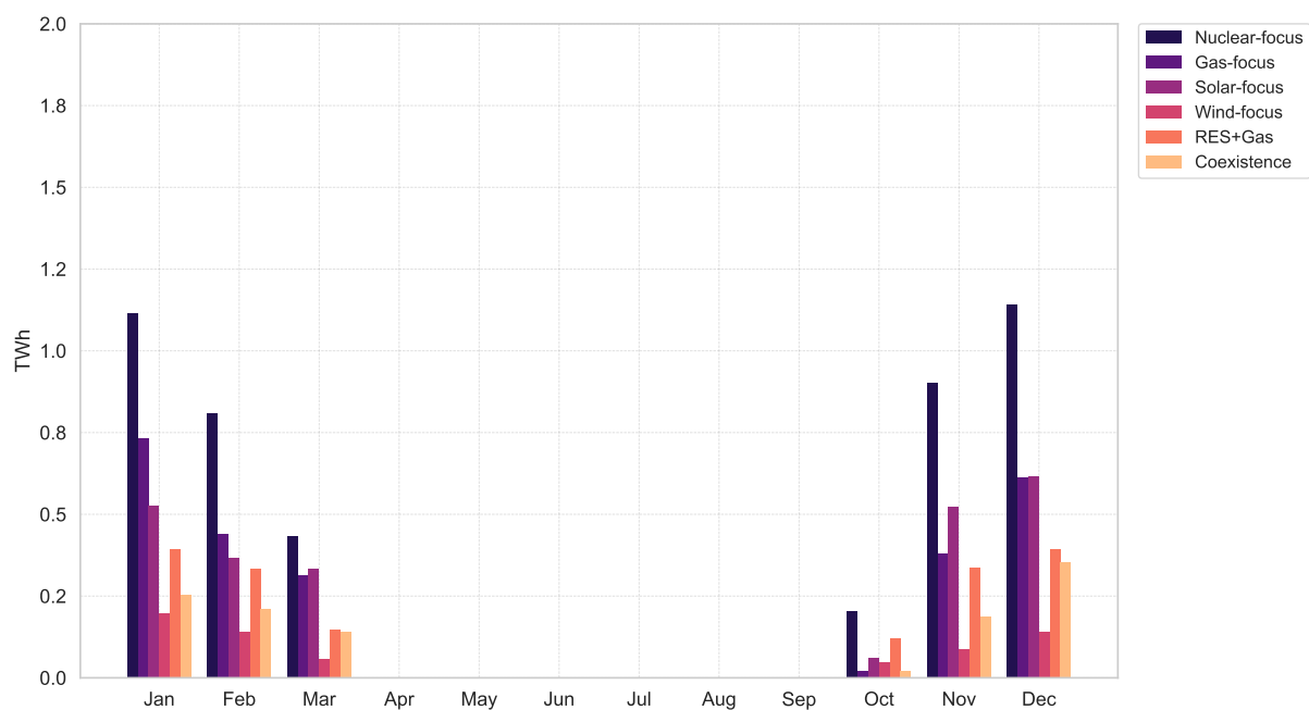
Figure 4.3.2: Monthly net imports of electricity in Switzerland in the quasi-autarky scenarios.
