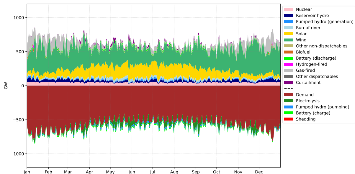
Figure 4.3.6: Annual energy dispatch (daily average) in Europe under the market-integrated scenario. The RES+Gas scenario is shown for illustrative purposes.
