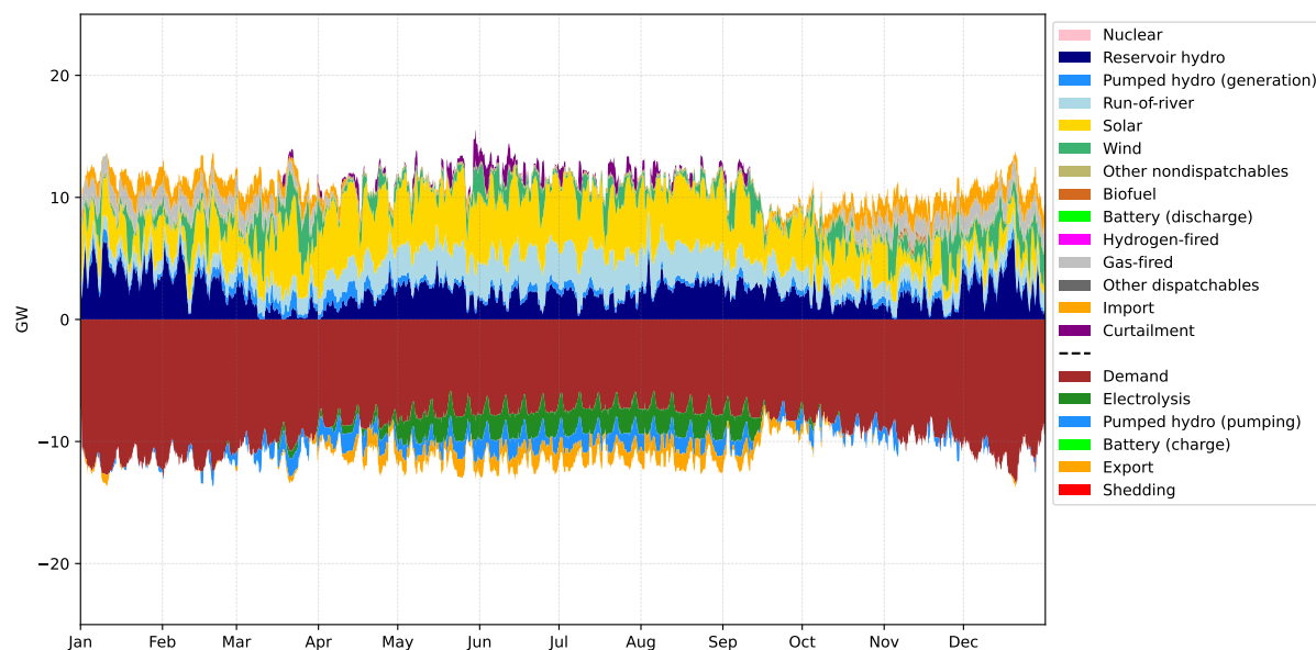
Figure 4.11.4: Annual energy dispatch (daily average) in Switzerland under the market-integrated scenario with NTCs reduced to 10%. The RES+Gas scenario in Switzerland is used for illustrative purposes.
