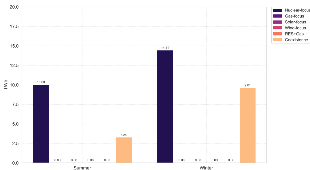
Figure 4.9.2: Seasonal nuclear plants production in the quasi-autarky scenarios.
