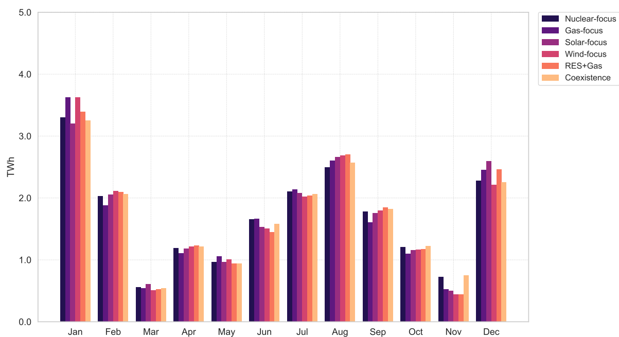
Figure 4.10.5: Monthly production of reservoir hydropower plants in Switzerland under the TYNDP market-integrated scenarios.
