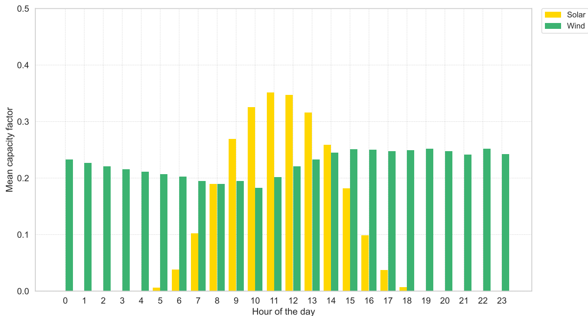
Figure 4.8.3: Mean capacity factors at hourly resolution in Switzerland for the weather year 2009 under Axpo assumptions.
