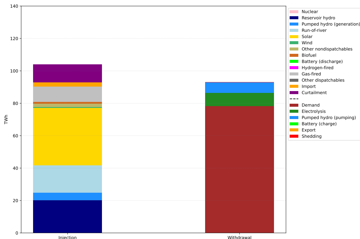
Figure 4.8.5: Annual energy dispatch (aggregation) in Switzerland under the Solar-focus quasi-autarky scenario.
