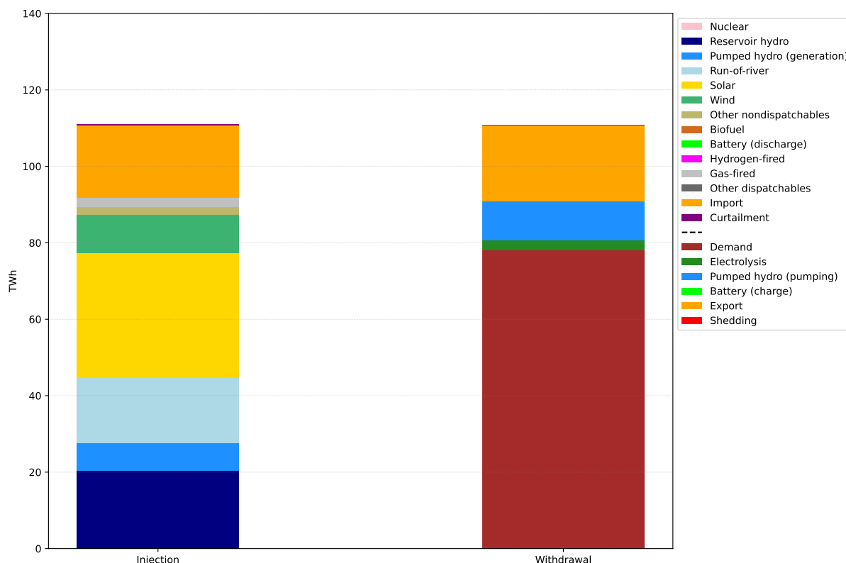
Figure 4.12.4: Annual energy dispatch (aggregated) in Switzerland under the market-driven scenario. The RES+Gas scenario in Switzerland is used for illustrative purposes.
