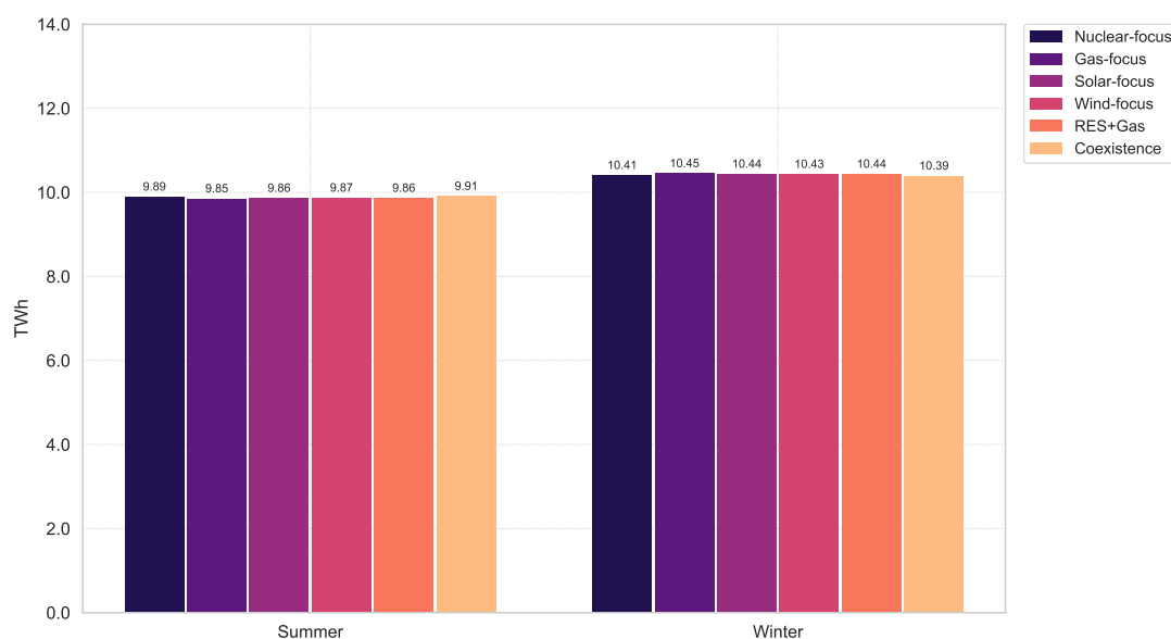
Figure 4.4.1: Seasonal production of reservoir hydropower plants in Switzerland under the quasi-autarky scenarios.
