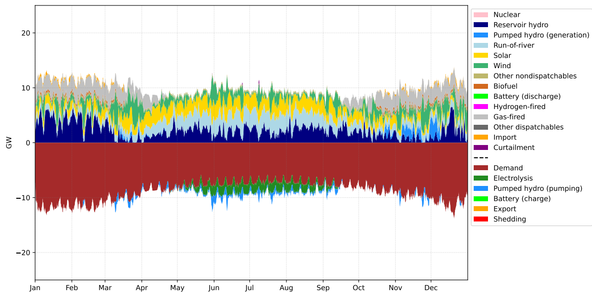
Figure 4.8.6: Annual energy dispatch (daily average) in Switzerland under the Wind-focus quasi-autarky scenario.
