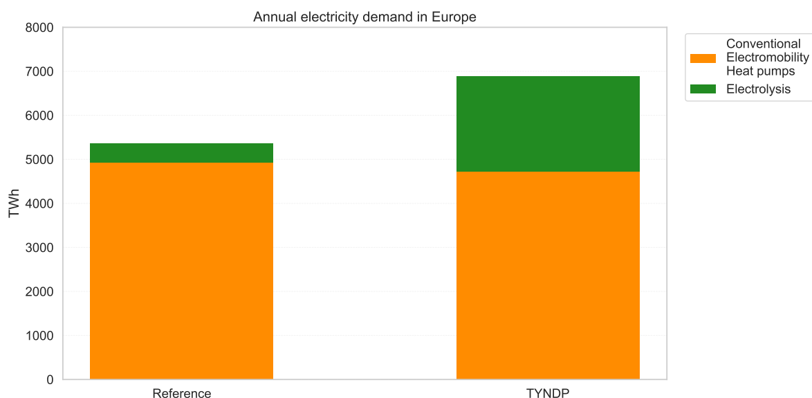
Figure 3.2.2: Final annual electricity demand in Europe in 2050 in the reference Axpo scenario and the selected TYNDP scenario.
