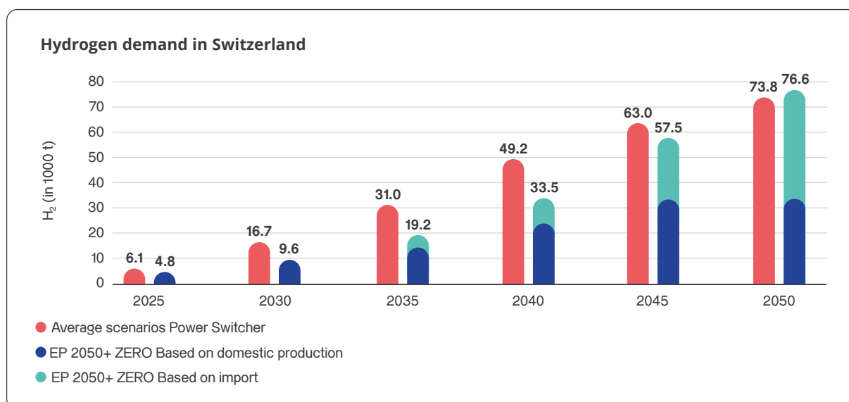
Figure 5: Modelled hydrogen demand in Switzerland. Comparison of Axpo Power Switcher** scenarios and Energy Perspectives 2050+ 7 study.
